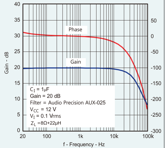
GAIN/PHASE vs FREQUENCY
