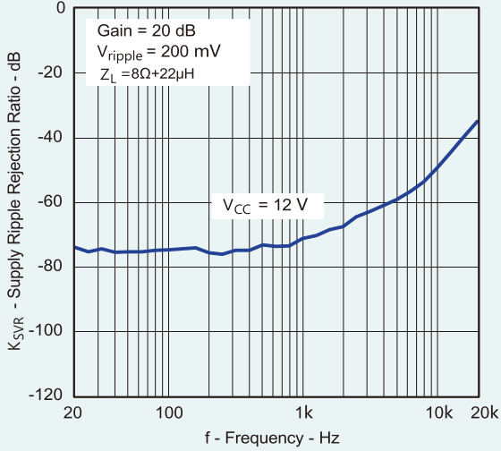
SUPPLY RIPLE REJECTION RATIO vs FREQUENCY
