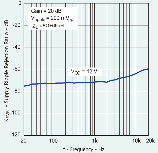
SUPPLY RIPLE REJECTION RATIO vs FREQUENCY
