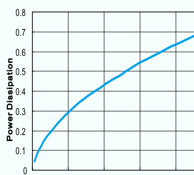
Power Dissipation vs. Output Power SE mode, 5V, f=1 kHz, RL=32 Ohm
