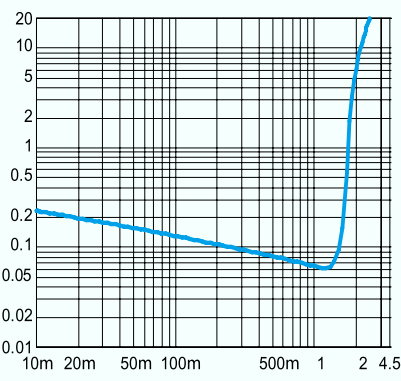
THD+N vs. Output Power BTL mode, 5V, 40Ohm, f=1 kHz
