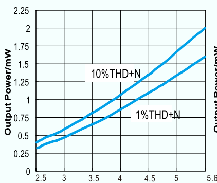
Output Power vs. Power Supply BTL mode, f=1 kHz, RL=8 Ohm
