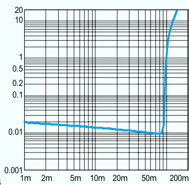
THD+N vs. Output Power SE mode, 5V, 32Ohm, f=1 kHz
