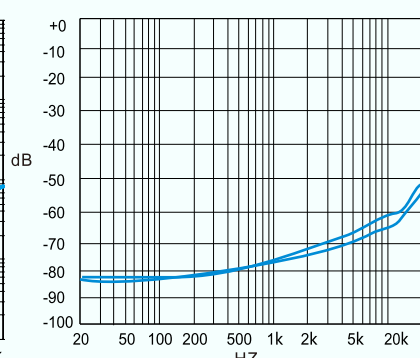
PSRR vs. Freq BTL mode, 5V, 8Ohm, 200mVpp Input terminated
