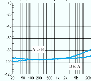
Crosstalk BTL mode, 3V, 8Ohm, Po=0.3W
