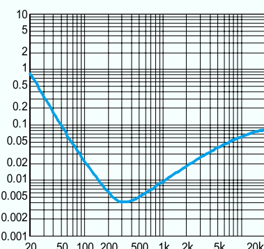
THD+N vs. Frequency SE mode, 5V, 32Ohm, Po=70mW
