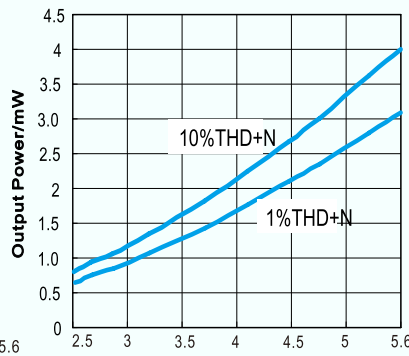
Output Power vs. Power Supply BTL mode, f=1 kHz, RL=4 Ohm
