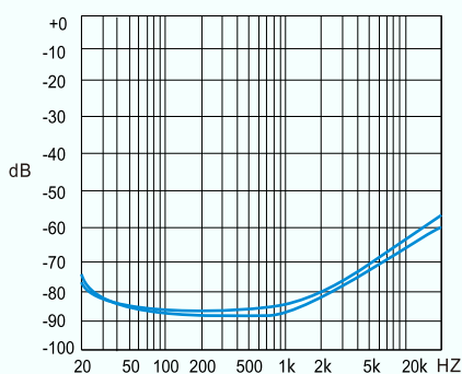
PSRR vs. Freq SE mode, 5V, 32Ohm, 200mVpp Input terminated
