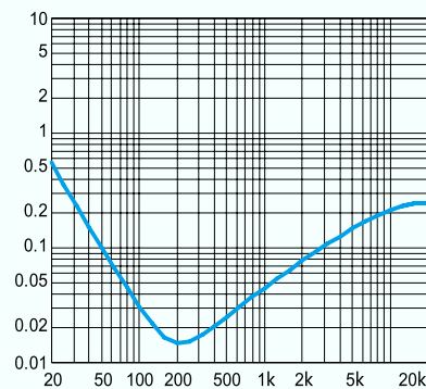
THD+N vs. Frequency BTL mode, 5V, 8Ohm, Po=800mW
