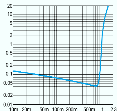
THD+N vs. Output Power 5V, 8Ohm, BTL at f=1 kHz
