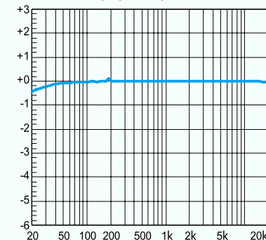
Frequency Response BTL mode, 5V, 8Ohm
