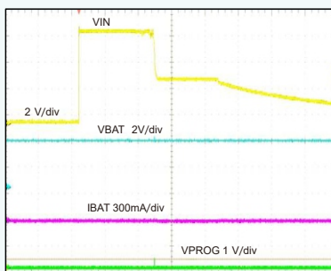
Hot Plug OVP7-VA adaptor
