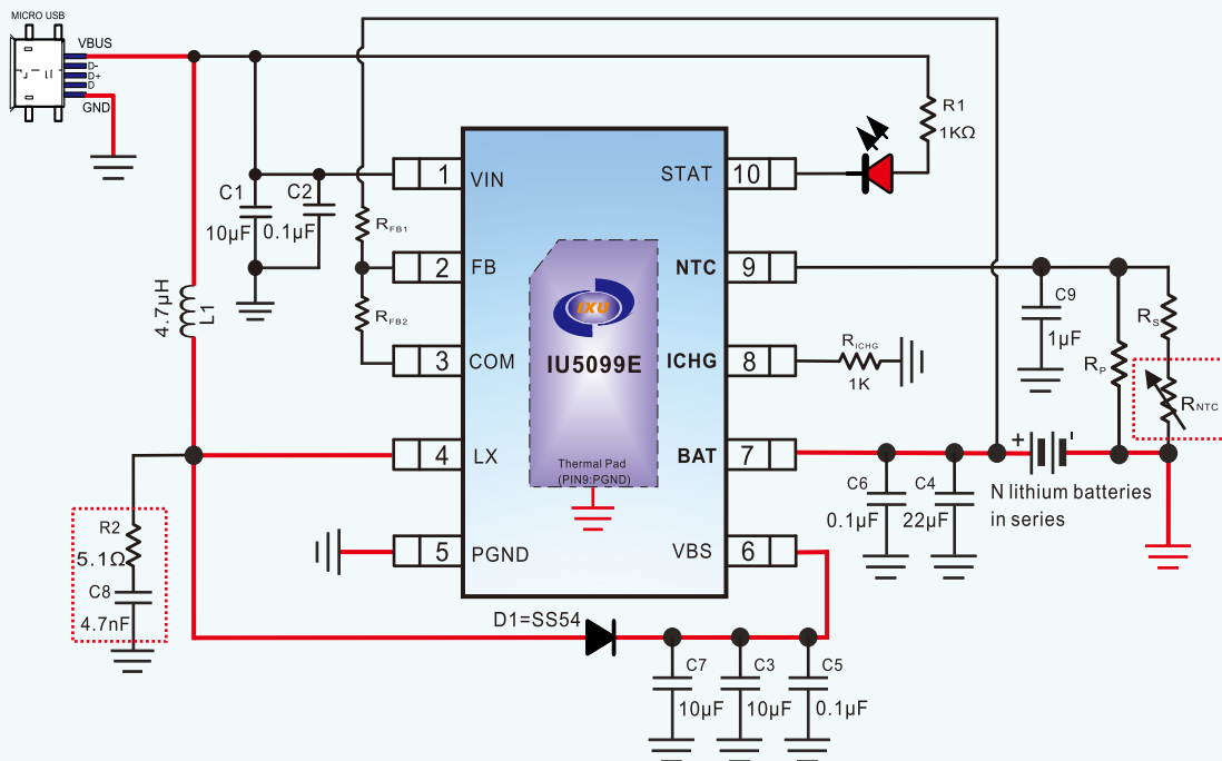
IU5099E Application Circuit
