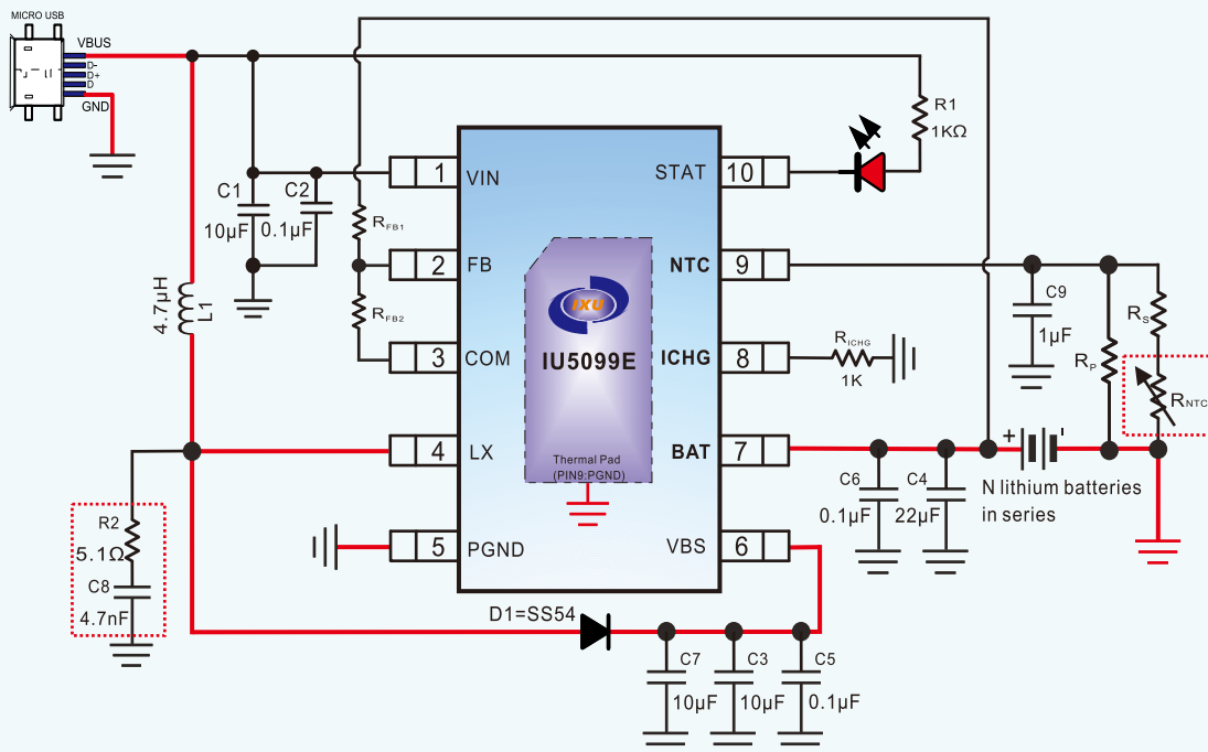
IU5099E Application Circuit
