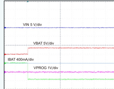
6- \Omega resistor at OUT, No input, V_{BAT} = 3.7\text{ V} Battery PlugIn
