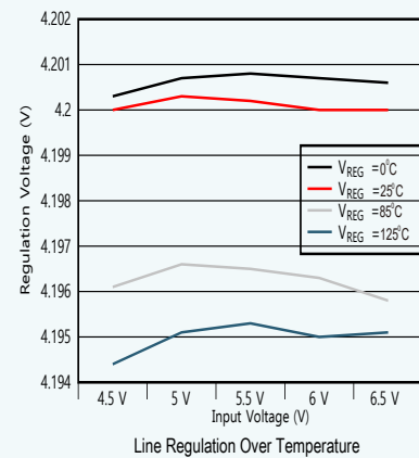
Line Regulation Over Temperature
