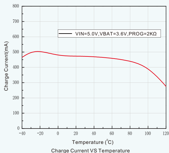
Charge Current VS Temperature
