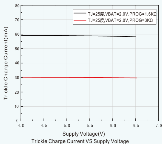
Trickle Charge Current VS Supply Voltage
