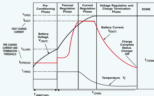
Charging Profile With Thermal Regulation
