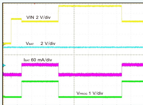
V IN 0V-5V-7V-5V t-time -50 ms/div OVP from Normal Power-Up Operation
