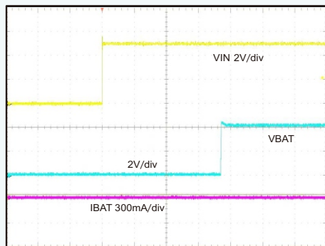
No Battery, No Load t-time - 5 ms/div Power Up Timing
