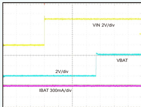
No Battery, No Load t-time - 5 ms/div Power Up Timing
