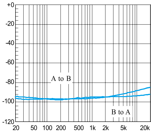
Figure 39. Crosstalk BTL mode, 6V, 8Ω, Po=1W
