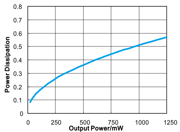
Figure 44. Power Dissipation vs. Output Power BTL mode, 5V, f=1 kHz, RL=8Ω, THD+N≤1%
