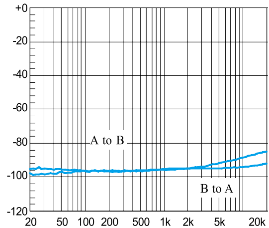
Figure 41. Crosstalk BTL mode, 3V, 8Ω, Po=0.3W
