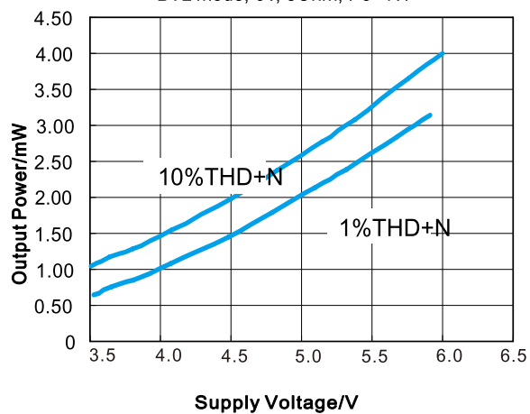
Figure 43. Output Power vs. Power Supply BTL mode, f=1 kHz, RL=8 Ω
