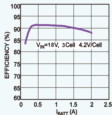
Efficiency Curve
