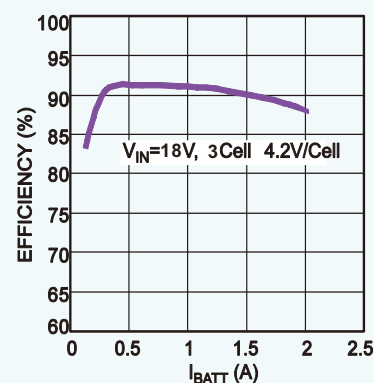
Efficiency Curve
