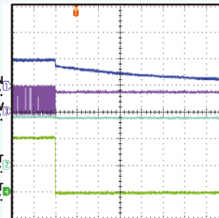
Power OFF
