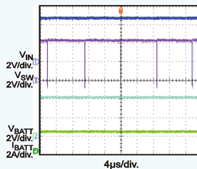
Power OFF
