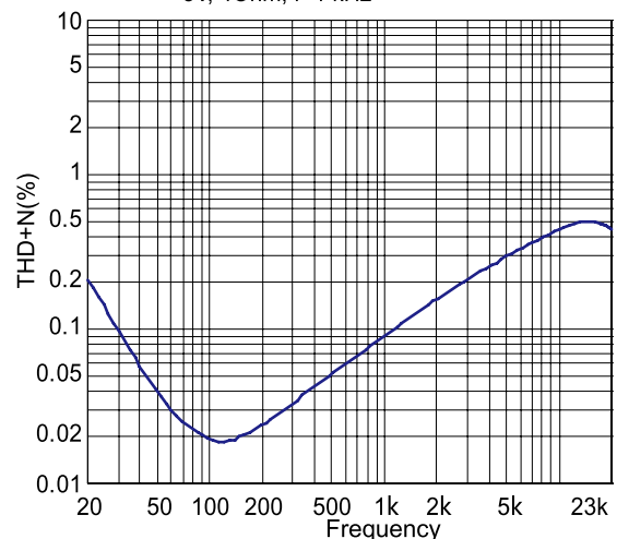
THD+N vs. Frequency 3V, 40hm, Po=500mW
