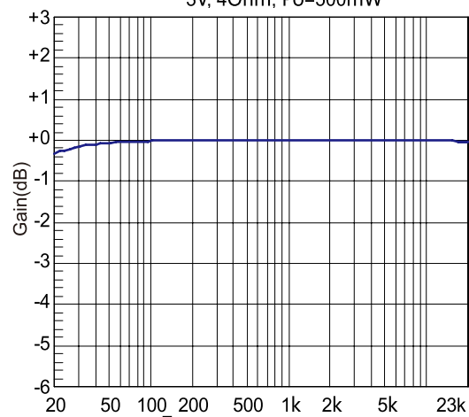
Frequency Response 3V, 40hm
