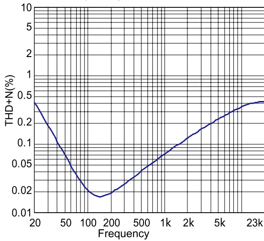
THD+N vs. Frequency 5V, 40hm, Po=1W
