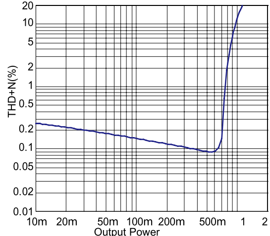
THD+N vs. Output Power 3V, 40hm, f=1 kHz
