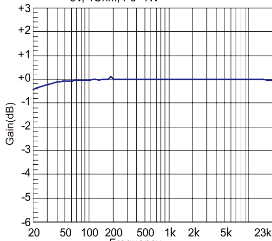
Frequency Response 5V, 40hm
