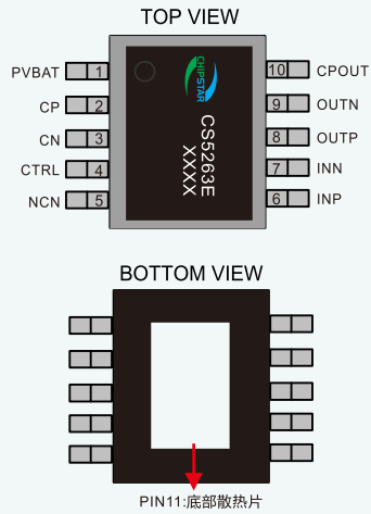
CS5263E(ESOP10 PACKAGE)
