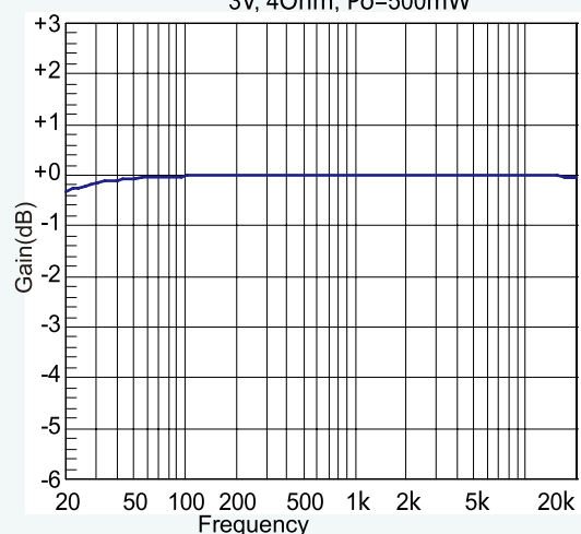
Frequency Response 3V, 4Ohm
