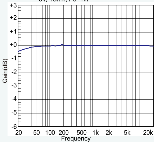
Frequency Response 5V, 4Ohm
