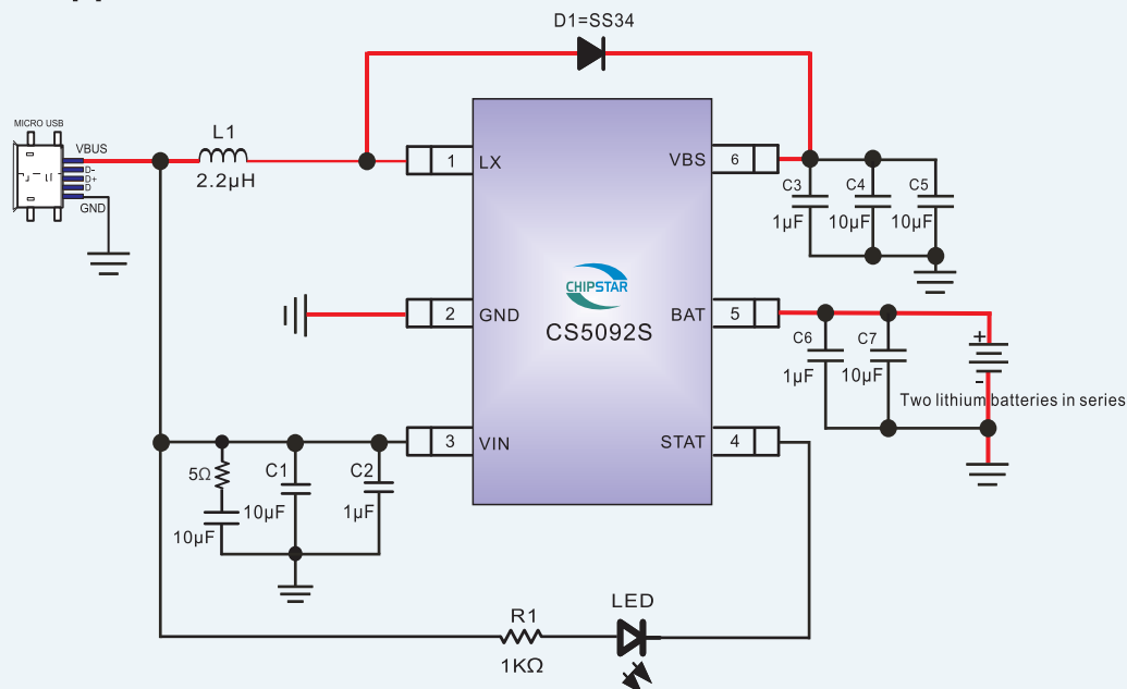
CS5092S Application Circuit
