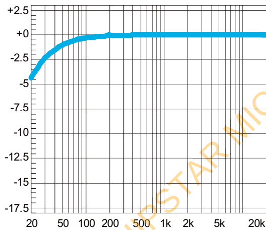
Frequency Response SE mode, 6V, 32Ohm
