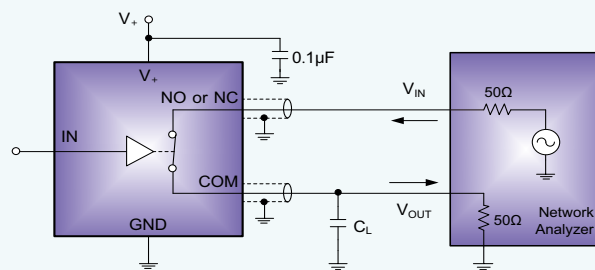
Test Circuit 3. -3dB Bandwidth
