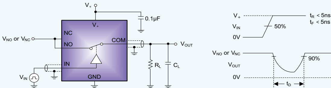
Test Circuit 5. Break-Before-Make Time Delay ( t_D )
