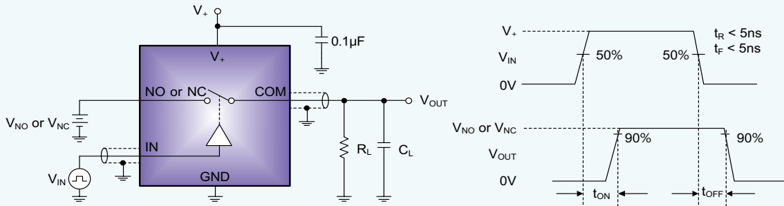
Test Circuit 4. Switching Times
