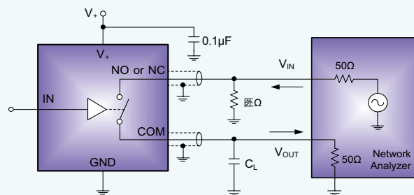
Test Circuit 2. Off Isolation
