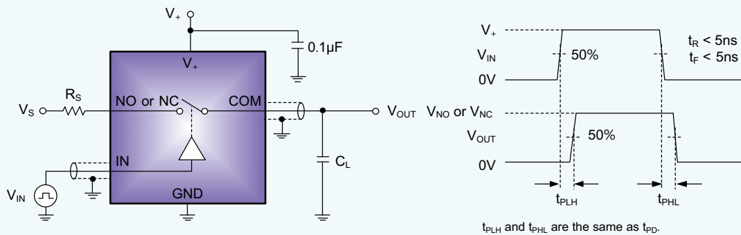
Test Circuit 6. Propagation Delay Time ( t_{PD} )
